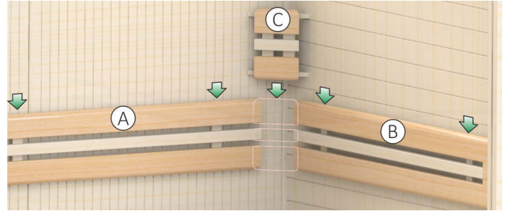
Figure 13. Installing Backrests
