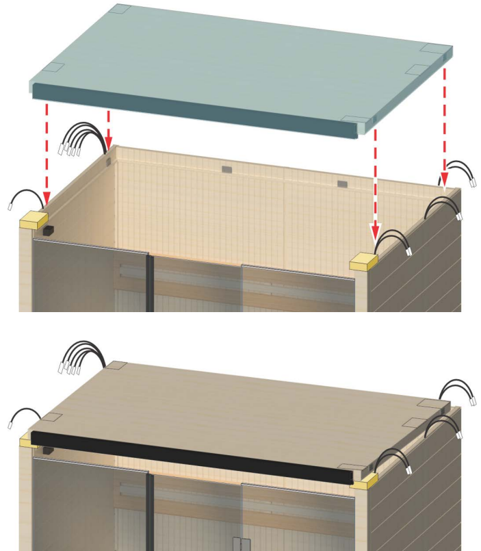
Figure 20. Preparing the Ceiling
