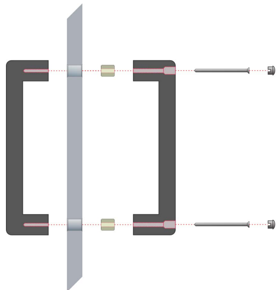
Figure 18. Installing Door Handle
