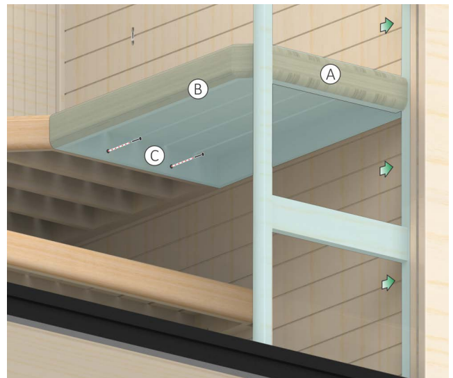
Figure 11. Installing Front Edge Trim
