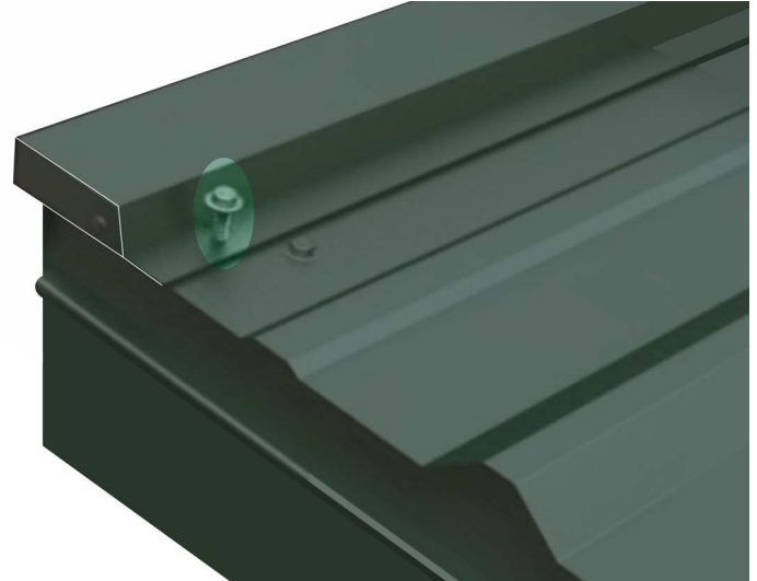
Figure 50. Attaching the Side Fascia
