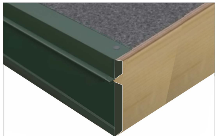
Figure 40. Applying Lower Rear Fascia
