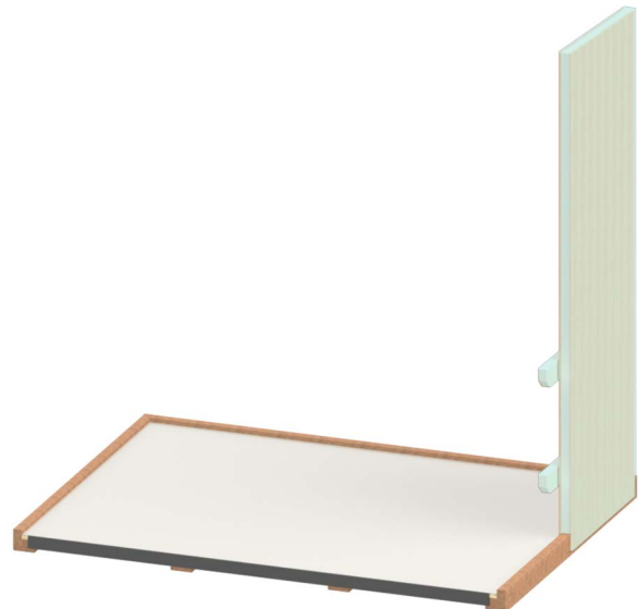
Figure 4. Installing #2 Wall Section
