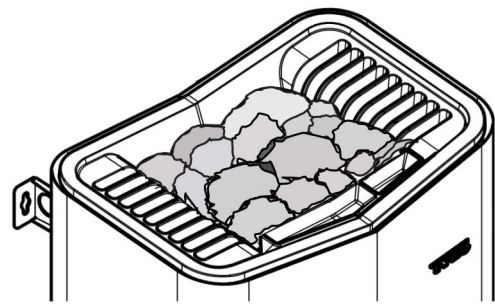
Figure 60. Placing Rocks on Top of Elements
