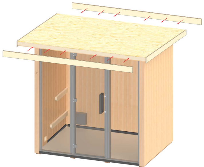
Figure 22. Installing Front and Back Wood Fascia
