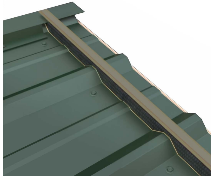
Figure 51. Applying Polyethylene Closure and Tape
