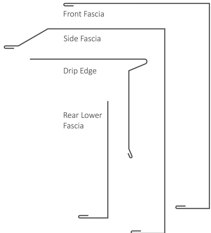
Figure 37. Metal Fascia Profiles
