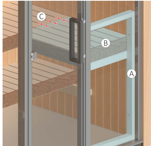
Figure 29. Installing Armrest and Return Bench
