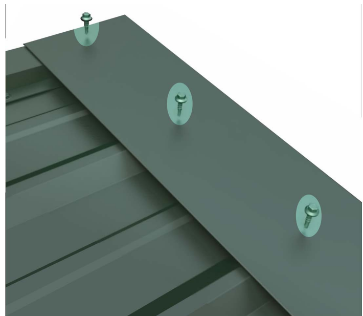
Figure 53. Attaching Front Edge Cap
