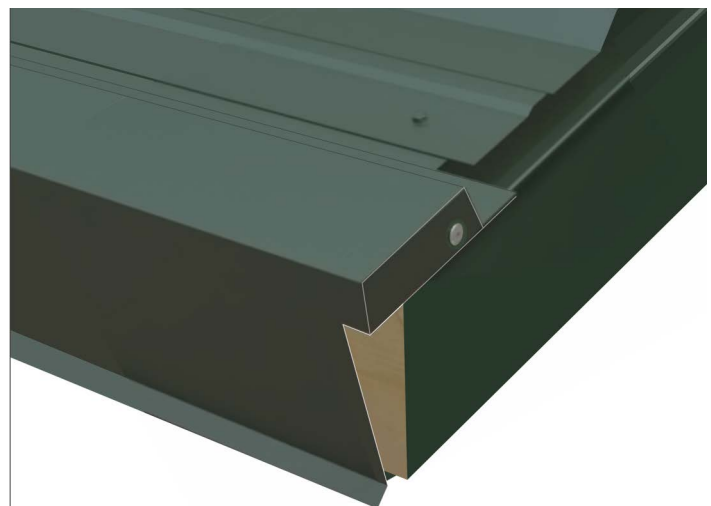
Figure 49. Ends Folded and Riveted
