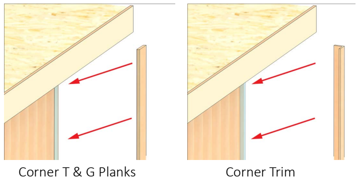
Figure 23. Installing Planks and Trim
