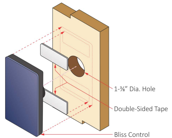
Figure 55. Mounting the Control
