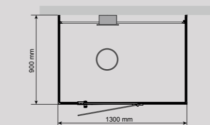
VISTA DCO 130 LEFT Size: D 900 x W 1 300 mm
