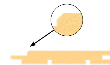
1. SAUNA PANEL STP PROFILE
