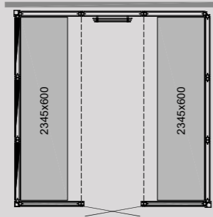
PANACEA 2525 2B 2525 x 2525 x 2090 mm
