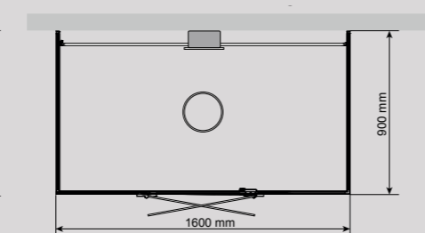
VISTA DCO 160 (LEFT & RIGHT) Size: D 900 x W 1 600 mm
