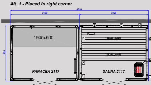
TWIN PANACEA 2117 Size: D 1725 x W 4254 mm
